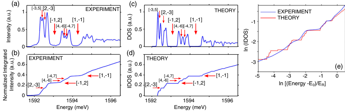
FIG. 4 (color online). (a) Measured total (angularly integrated) emission spectrum I(\epsilon) of the quasiperiodic wire and (b) spectrally integrated emission intensity \int_{E_0}^{\epsilon} I(\epsilon') d\epsilon' (where E_0 is the lower energy state). Calculated normalized DOS (c) and IDOS (d). (e) Display of the log-periodic oscillations of the IDOS in a log-log plot of numerical (red) and experimental (blue) IDOS in the vicinity of E_0 (normalized to E_R = \hbar^2 \pi^2 / (8a^2 m_p) , with m_p the polariton mass).
